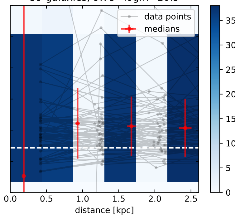
39 galaxies, 9.75 < \log m < 10.5
