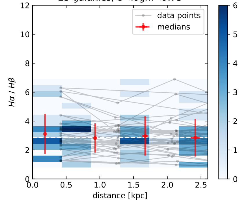
23 galaxies, 8 < \log m < 9.75
