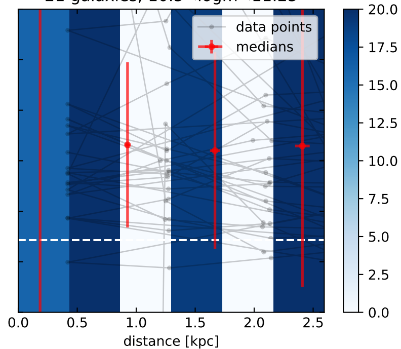
21 galaxies, 10.5 < \log m < 11.25
