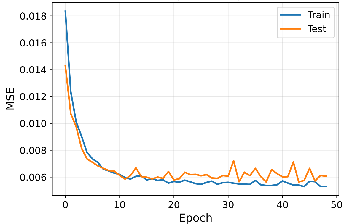
Axis Ratio (q): Training Curves
