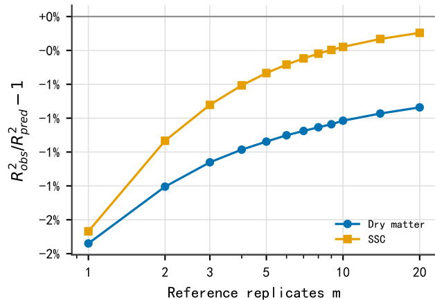
b Relative deviation shrinks with m
