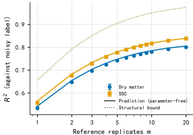
a Semi-synthetic: degradation under reference noise
