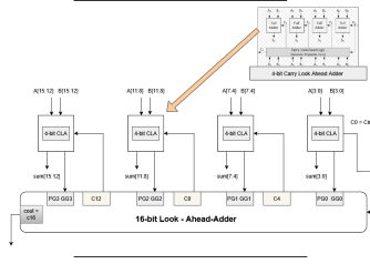
Fig. 3. 16-bit Carry Lookahead Adder
