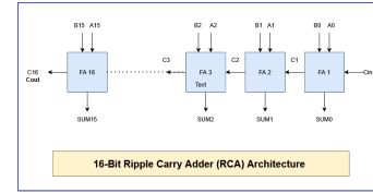
Fig. 2. 16-bit Ripple Carry Adder
