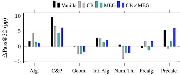
Fig. 3. Change in MATH-500 Pass@32 relative to the base model by subject, the macro gate's topics (mean over seeds).
