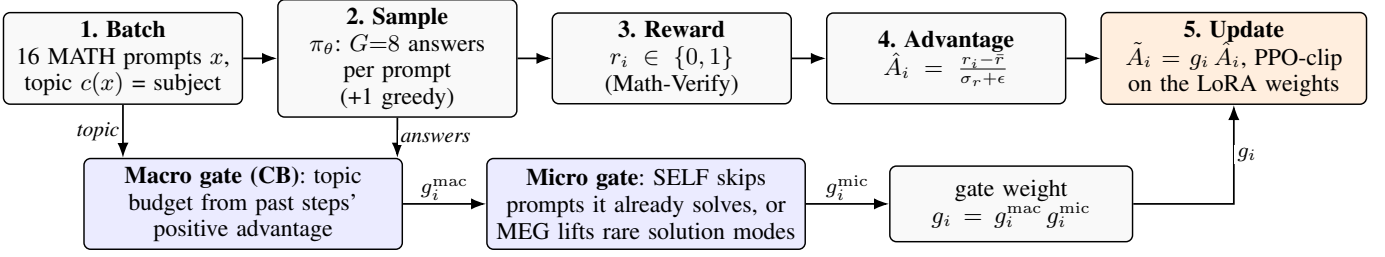
Fig. 1. One training step of gated GRPO. The macro gate knows each prompt’s topic and how much positive advantage that topic has absorbed in past steps; the micro gate sees the current group’s answers (and greedy answer). Their product scales the advantage. Vanilla GRPO sets both gates to 1.
