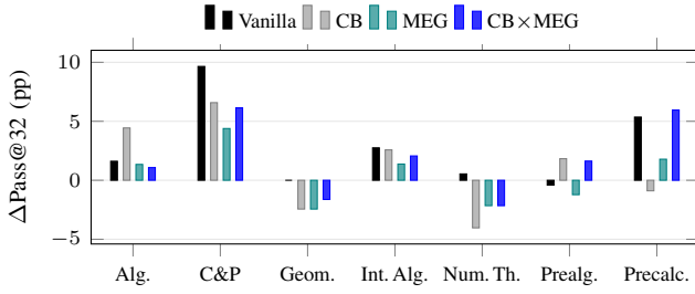
Fig. 3. Change in MATH-500 Pass@32 relative to the base model by subject, the macro gate’s topics (mean over seeds).
