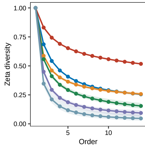
i. Primary common-n zeta diversity decay
