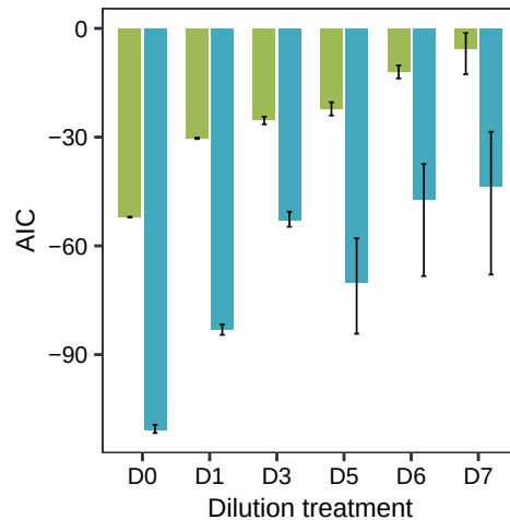
iii. Regression fitting to zeta decay
