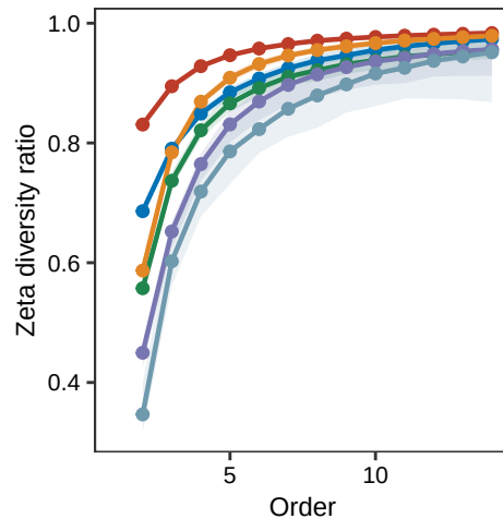
ii. Primary common-n zeta ratio
