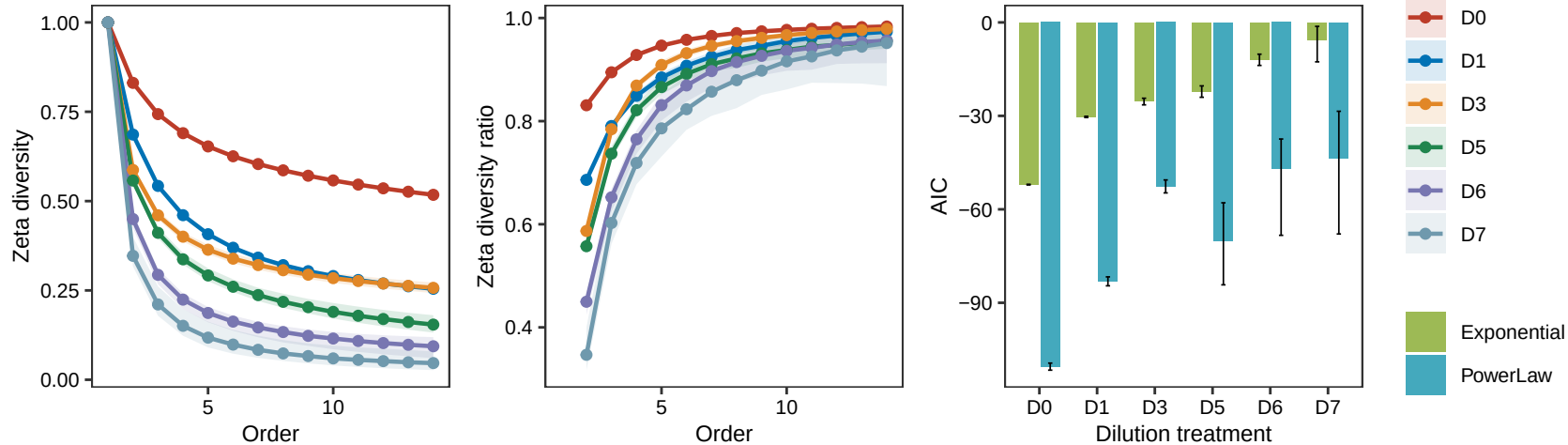
i. Primary common-n zeta diversity Primary common-n zeta ratio (in Reg 1) Regression fitting to zeta decay ( n = 14 )
