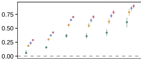
Median index of dispersion
