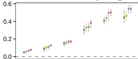
Non-normal OTUs (FDR q)
