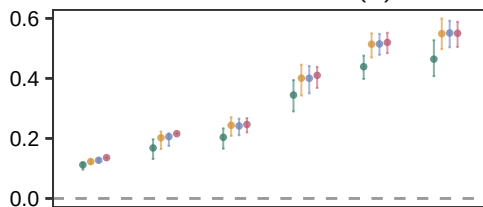
Non-normal OTUs (P)
