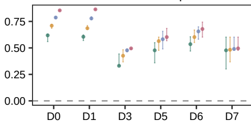
Median index of dispersion
