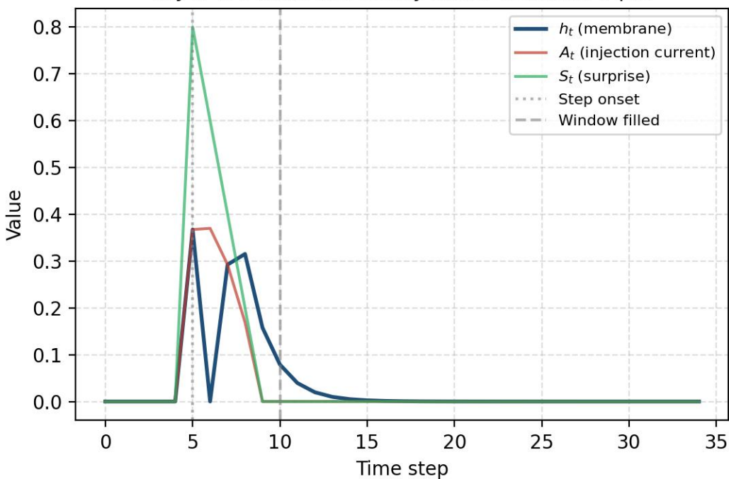
Layer 1: Membrane Decay under Constant Input
