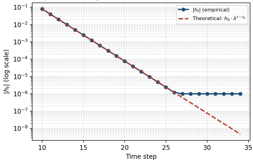
Exponential Decay Verification (mean ratio = 0.500, \lambda = 0.5 )
