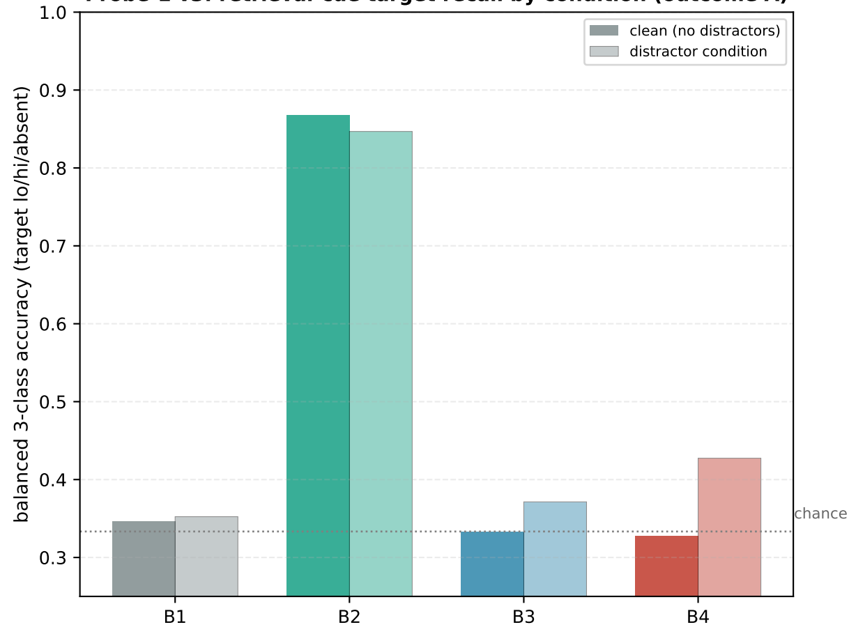
Probe-1 v3: retrieval-cue target recall by condition (outcome A)
