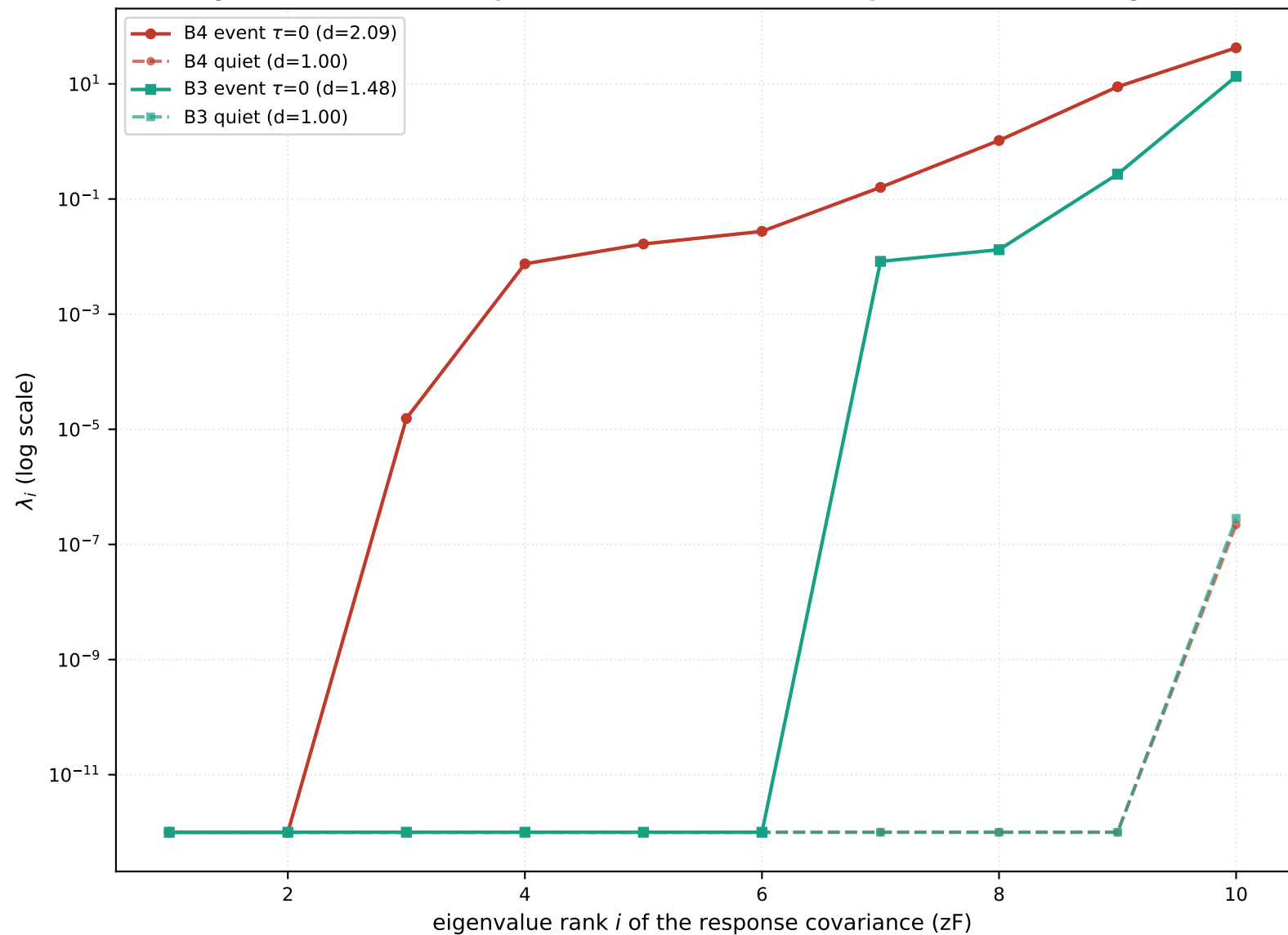
fig26 - Quiet vs event spectra: new directions vs amplification of existing ones
