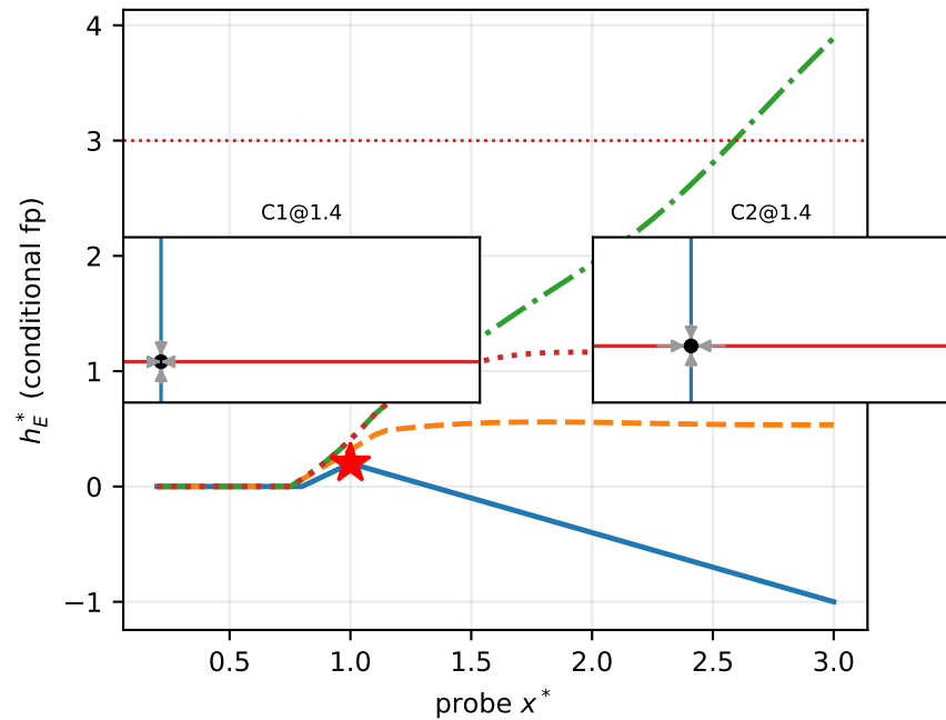
(b) Conditional Fixed-Context Phase Planes (nullclines = constant lines; NOT an autonomous 2-D portrait)
