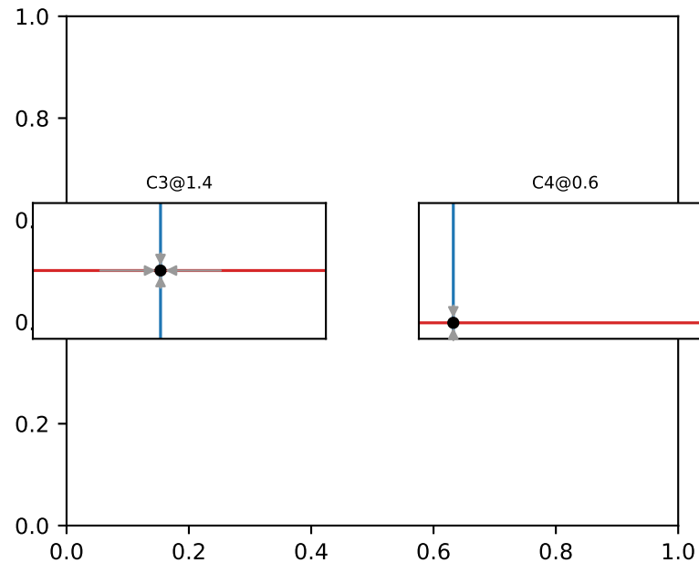
(b) Conditional Fixed-Context Phase Planes (nullclines = constant lines; NOT an autonomous 2-D portrait)
