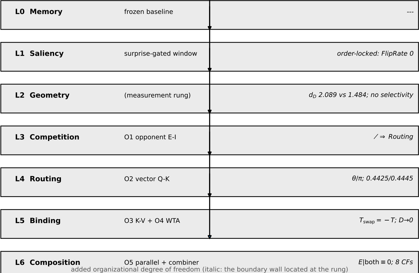
Figure 6 — The Unified Mechanistic Ladder of Dynamical Computation
