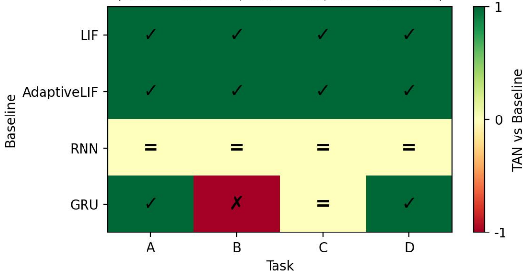
Win/Loss Heatmap: TAN vs each Baseline (Green = TAN wins, Yellow = tie, Red = TAN loses)
