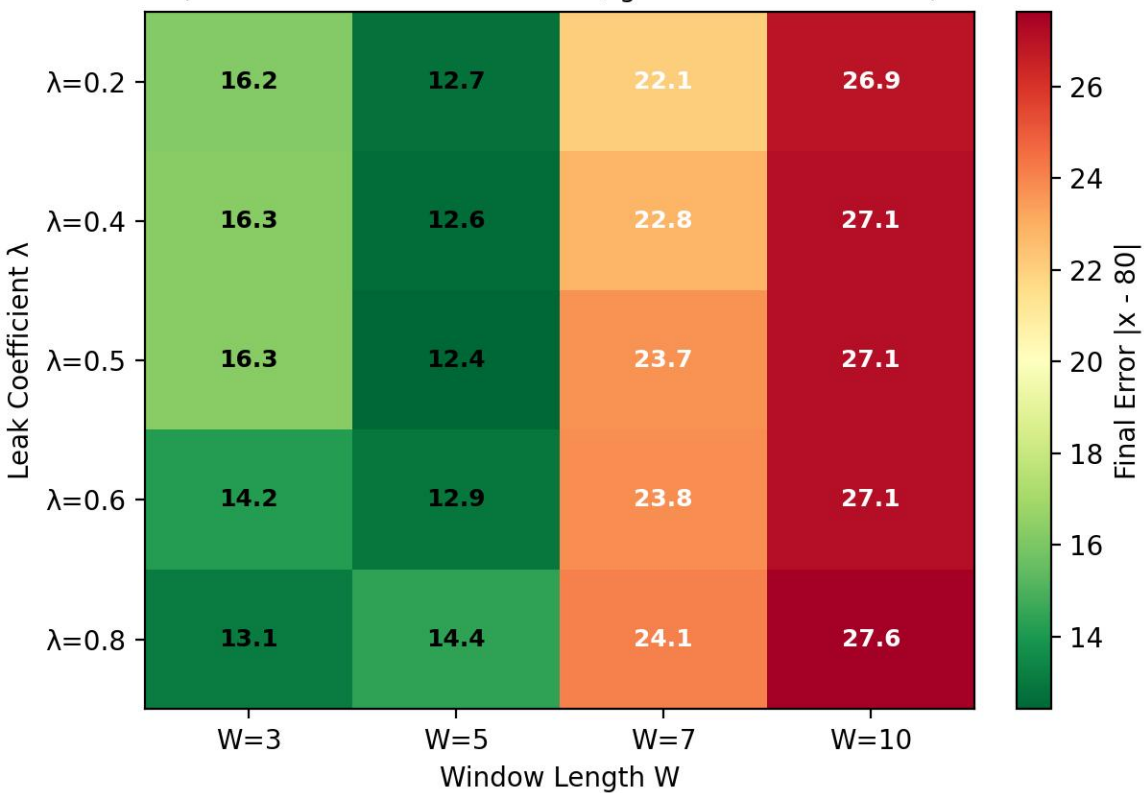
2D Interaction Sweep: \lambda \times W on Task D (mean final error over 20 seeds; green = lower = better)
