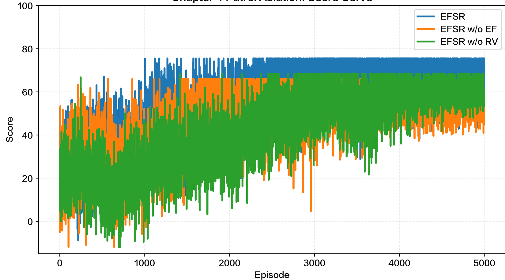
Chapter 4 Patrol Ablation: Score Curve
