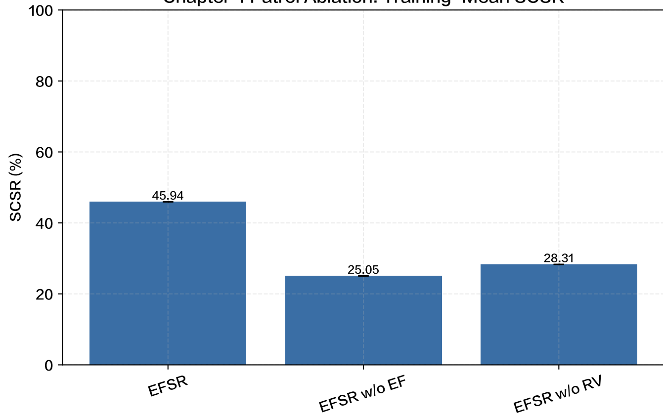
Chapter 4 Patrol Ablation: Training-Mean SCSR
