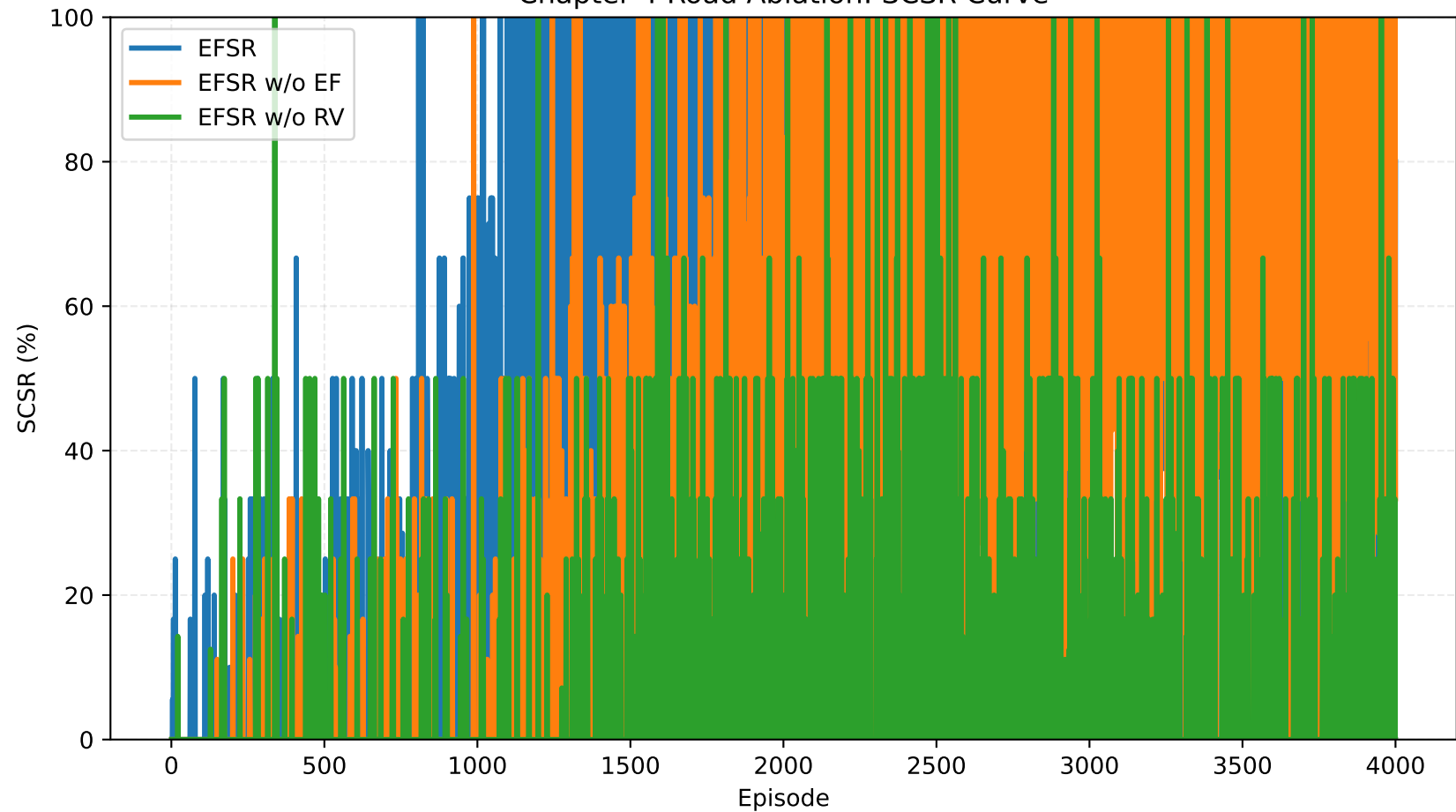
Chapter 4 Road Ablation: SCSR Curve
