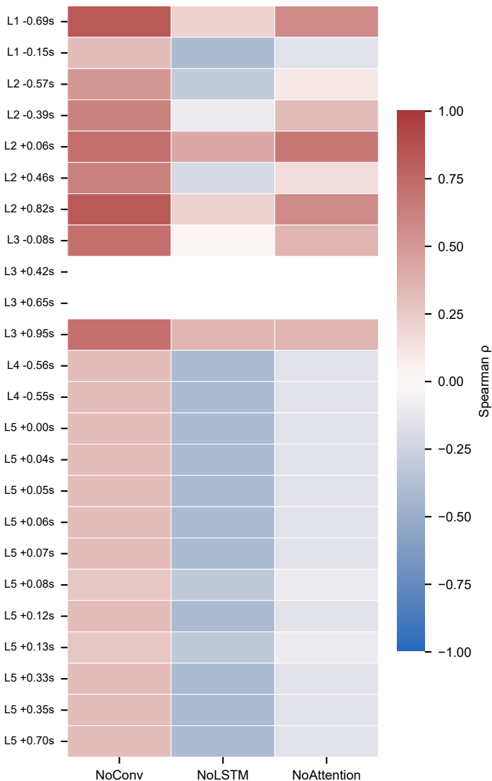
Similarity of 5-behavior \Delta Recall vectors
