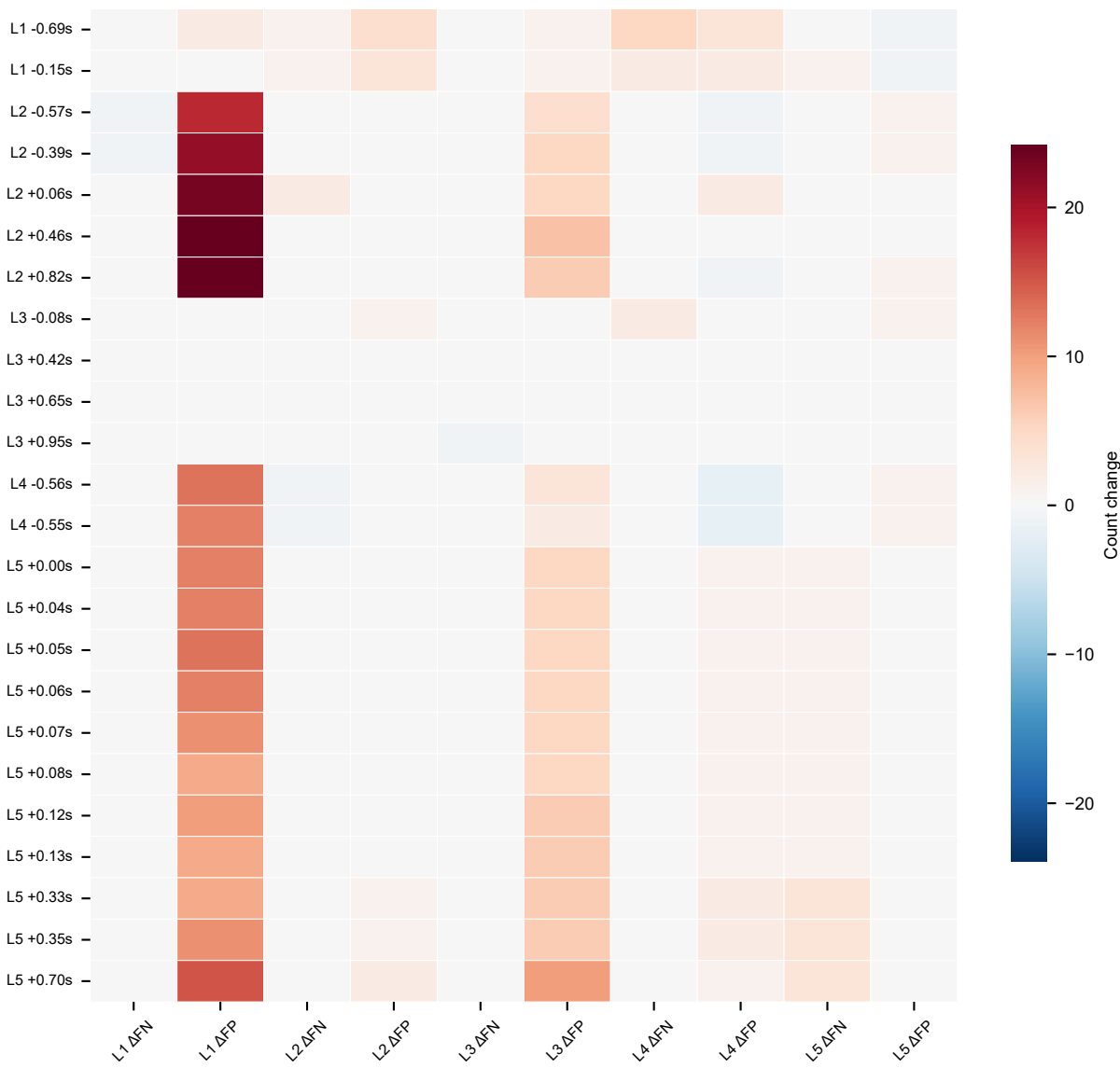
One-vs-rest error-count changes after data ablation
