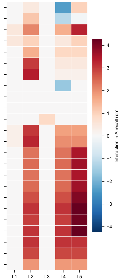
NoAttention
