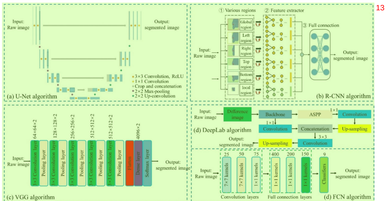
Fig. 9 Sketch maps of a U-Net (Siddique et al. 2021), b R-CNN (Zhang et al. 2018), c VGG (Zakaria and Hassim 2024), d DeepLab (Wang et al. 2021a, b, c) and e FCN (Dolz et al. 2018) algorithms
