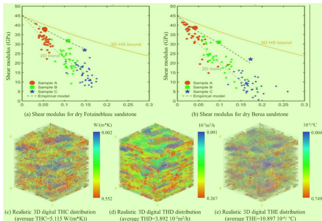
Fig. 13 Examples of petro-physical parameter evaluations (Saxena and Mavko., 2016; Zhao and Zhou 2021)
