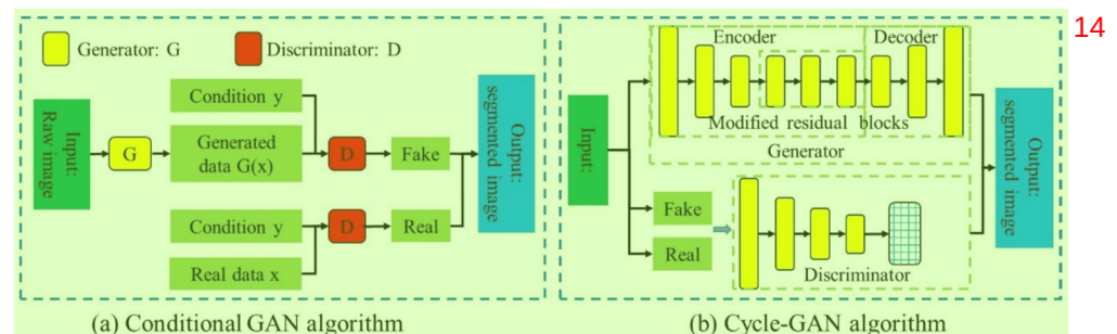
Fig. 11 Sketch maps of a conditional GAN and b cycle-GAN algorithms (Jin et al. 2023; Cho et al. 2020)
