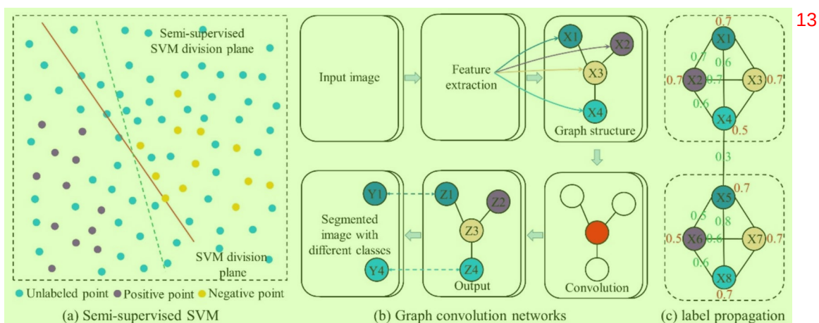
Fig. 5 Sketch maps of a Semi-supervised SVM, b Graph convolution networks, and c label propagation algorithms
