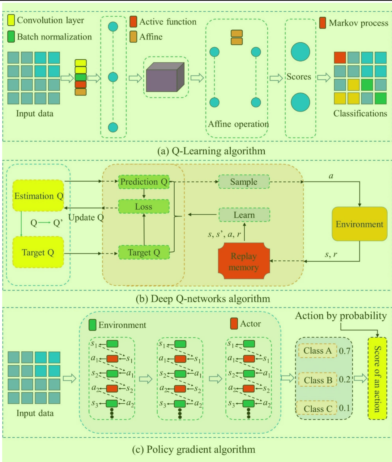
Fig. 6 Sketch maps of a Q-Learning, b Deep Q-networks, and c Policy gradient algorithms 2
