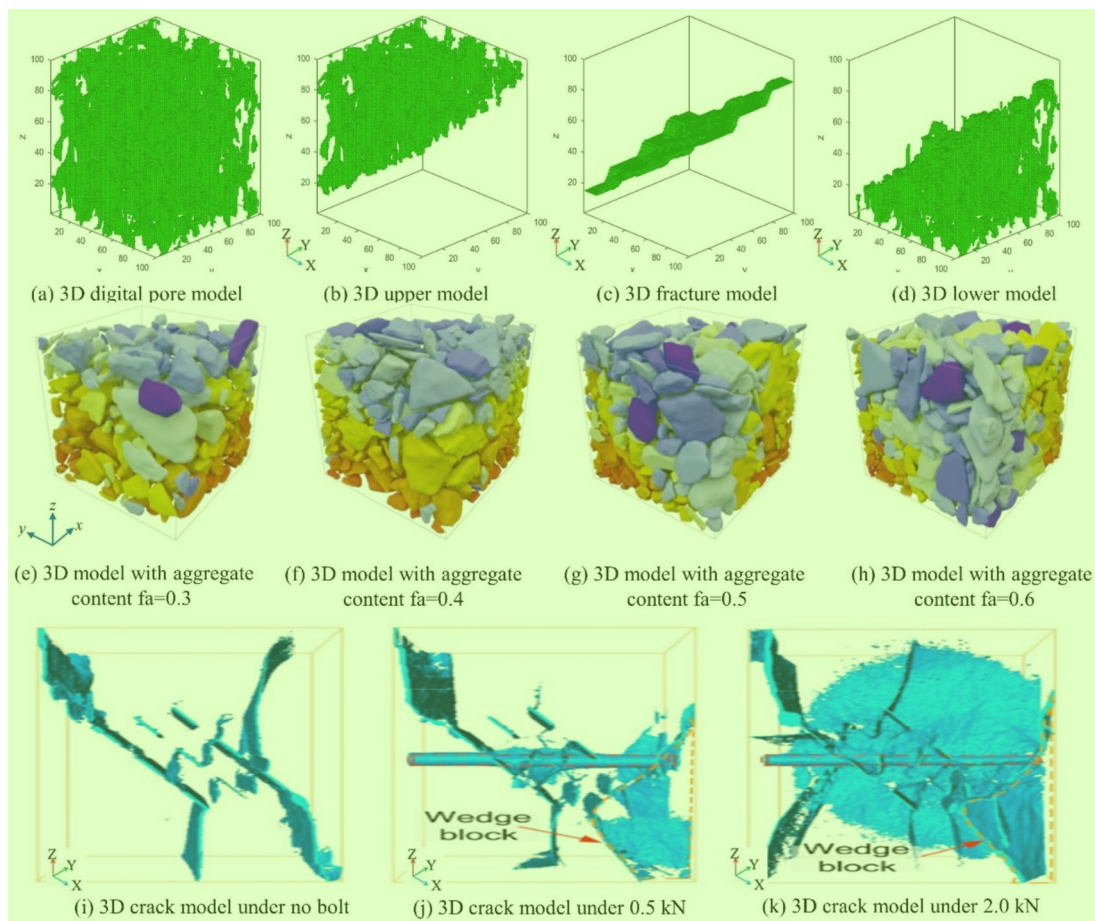
Fig. 14. 3D modes of various structures of rocks under different scales (Zhao and Zhou 2023a, b; Huang et al. 2023; Yang et al. 2020a, b)
