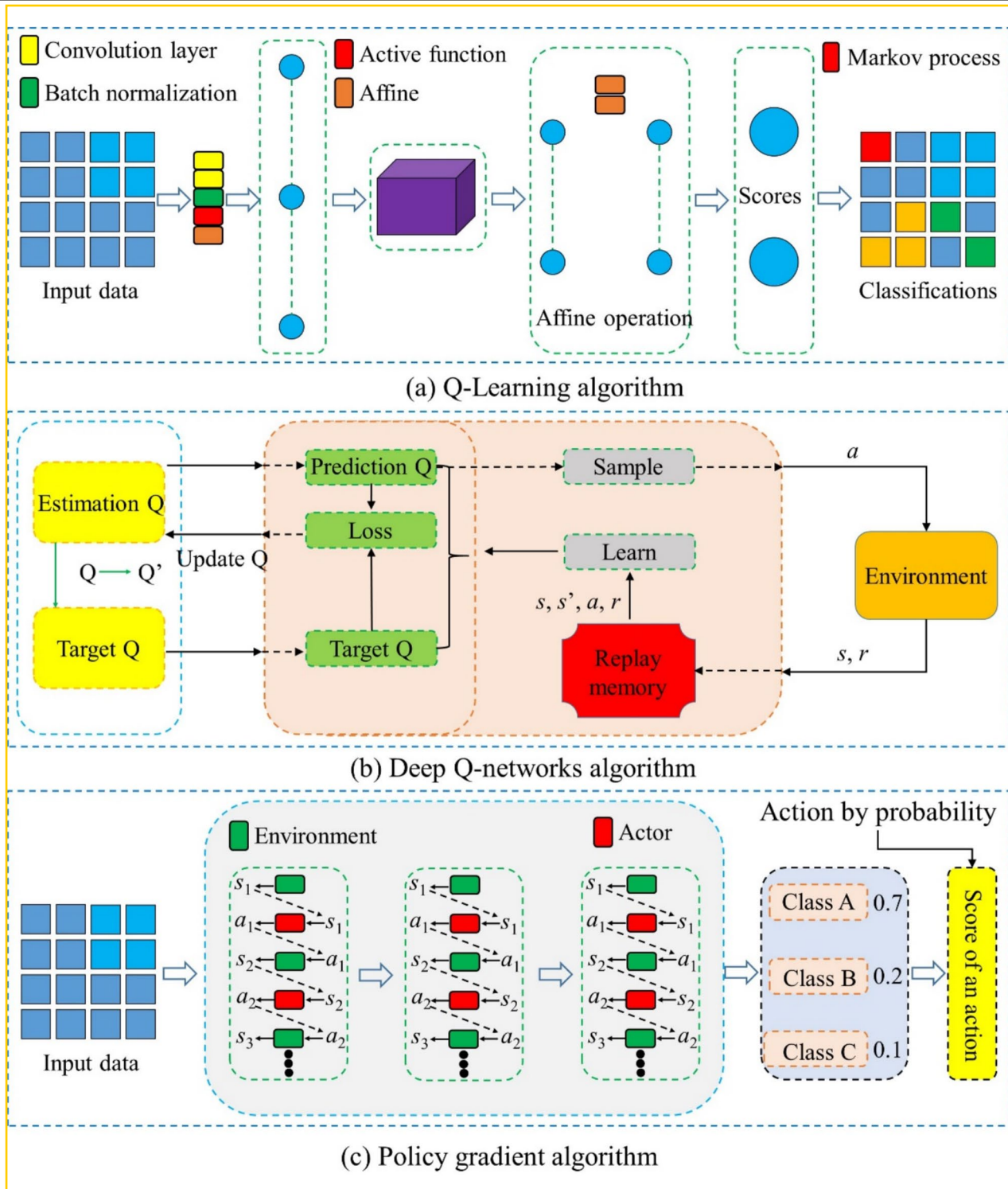
Fig. 6 Sketch maps of a Q-Learning, b Deep Q-networks, and c Policy gradient algorithms
