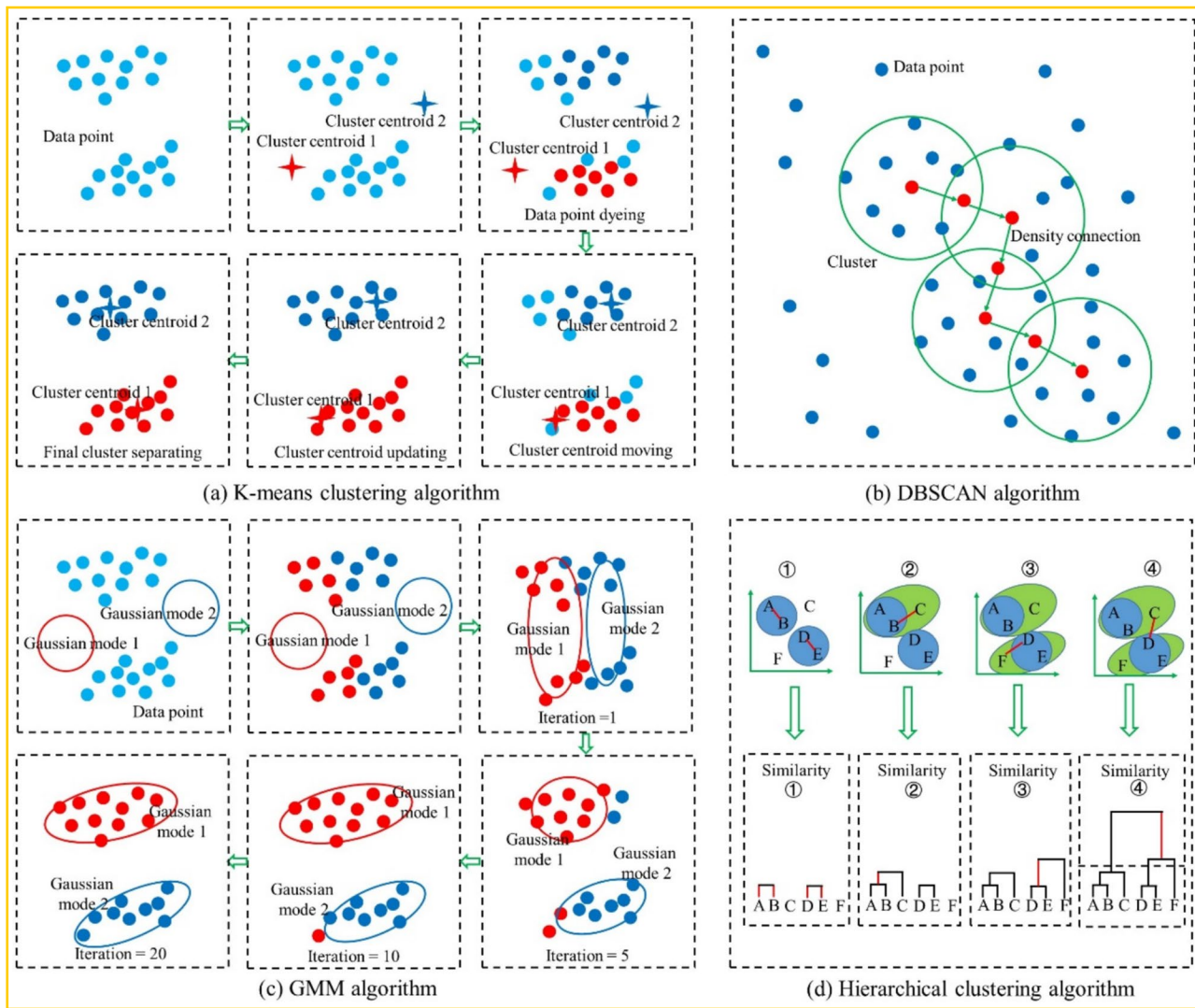
Fig. 4 Sketch maps of a K-means clustering algorithm, b DBSCAN algorithm, c GMM algorithm and d Hierarchical clustering algorithm
