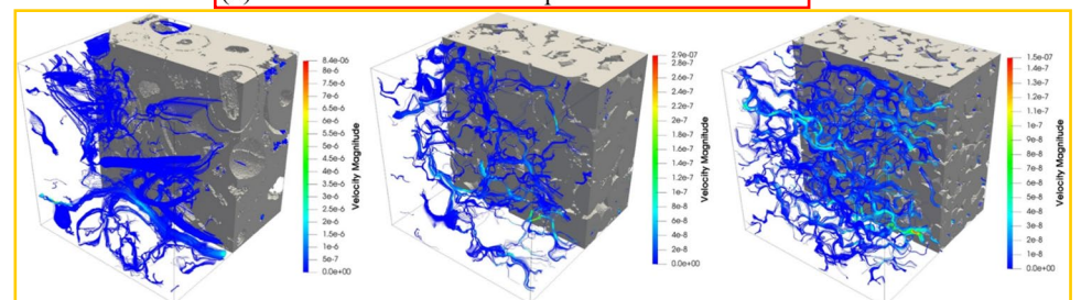
(b) Pore-scale permeability and fluid flow behaviors of rocks
