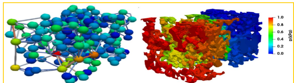
(a) Fluid flow behaviors in pore network of rocks
