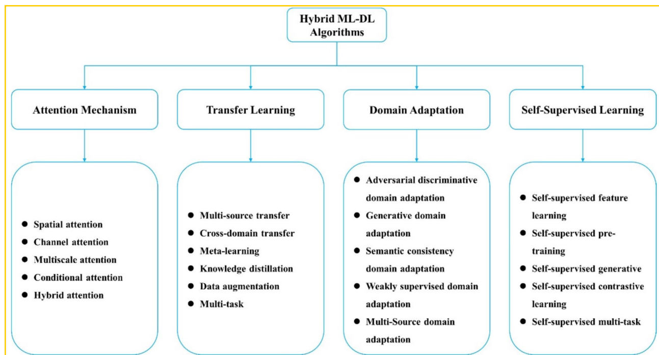
Fig. 12 Various hybrid ML-DL algorithms
