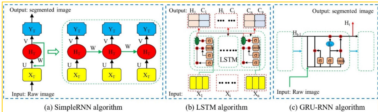
Fig. 10 Sketch maps of a SimpleRNN, b LSTM and c GRU-RNN algorithms (Kawakami 2008; Hochreiter and Schmidhuber 1997; Cho et al. 2014)
