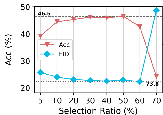
OCTMNIST
