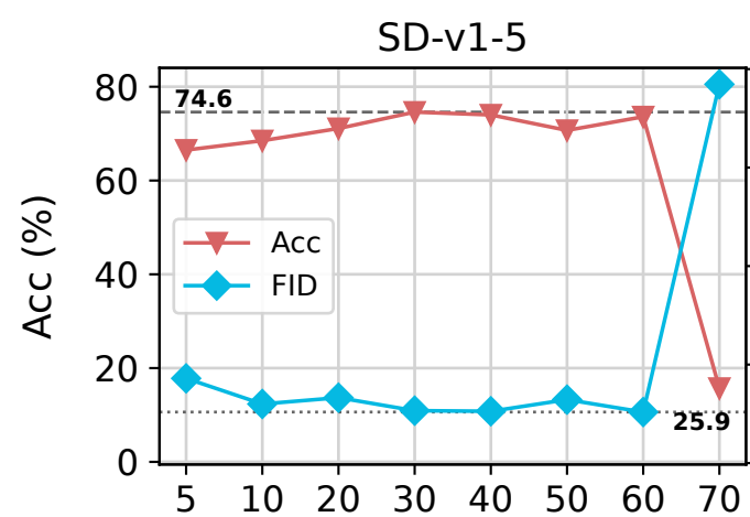
CIFAR-10
