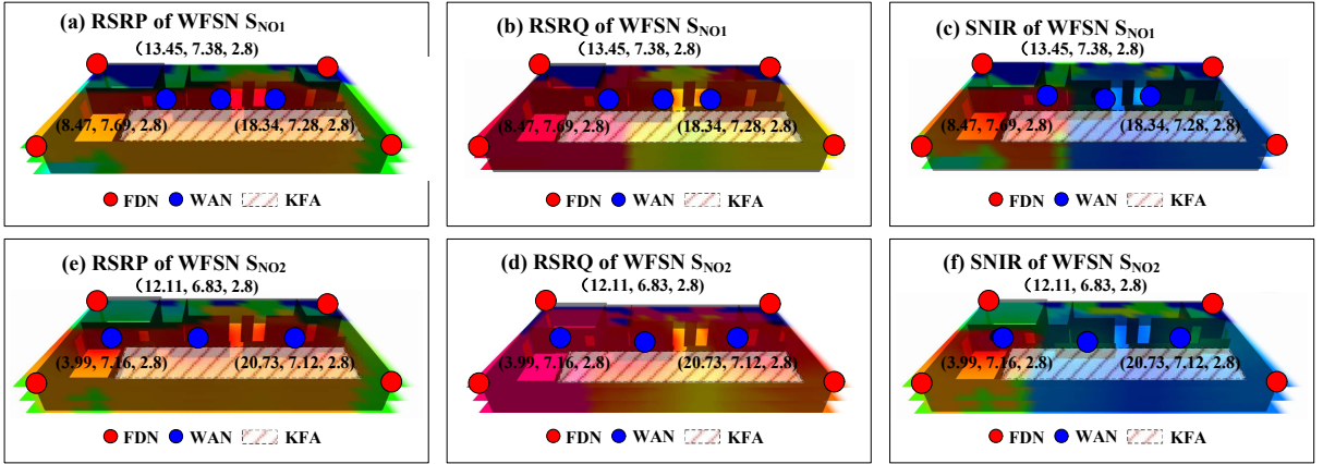
Fig. S2 Performance indicator values of the scheme based on numerical optimizations for the electrical substation
