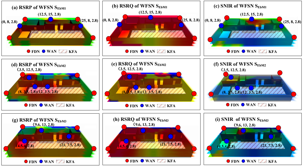
Fig. S1 Performance indicator values of the scheme based on expert-based methods for the electrical substation
