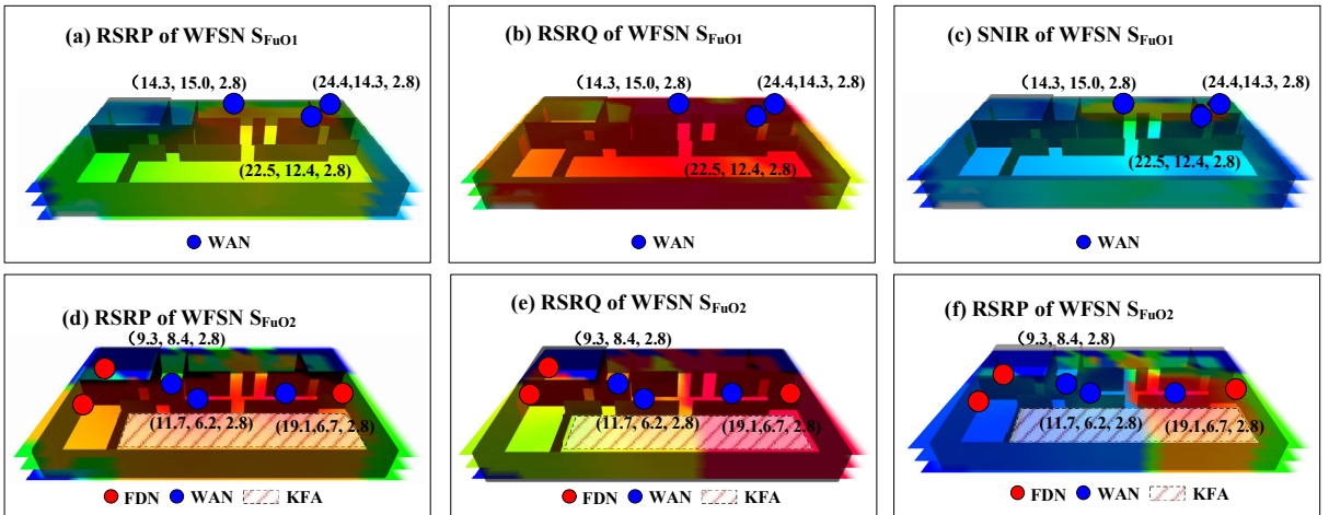
Fig. S3 Performance indicator values of the scheme based on FDN-unaware optimizations for the electrical substation
