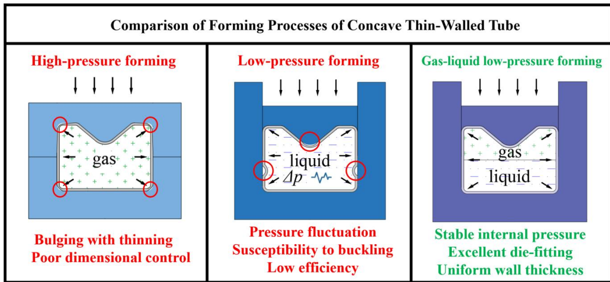
Fig. 1 Comparison of typical forming processes for complex concave thin-walled metal tubes
