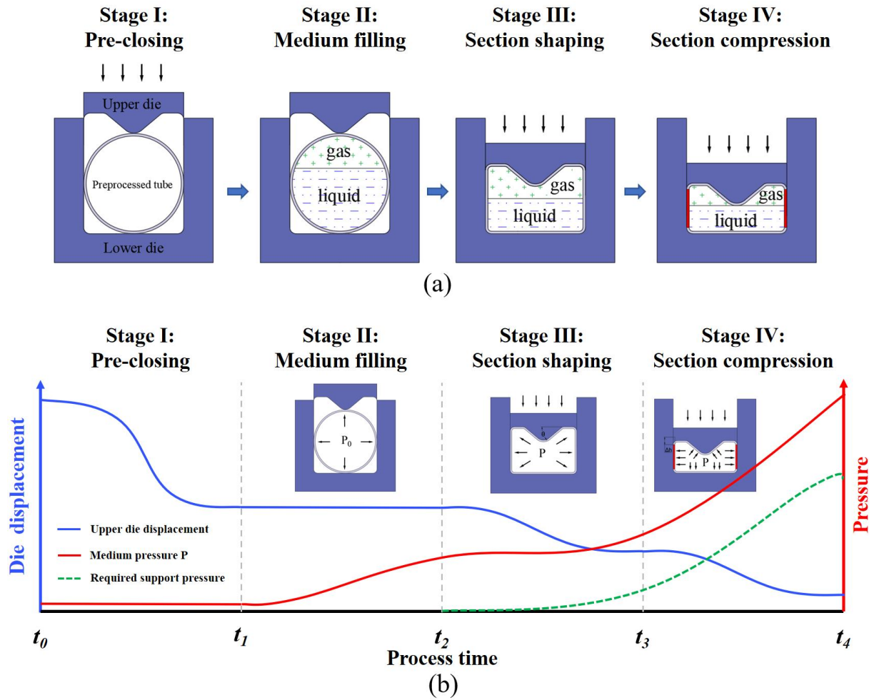
Fig. 2 The principle and typical deformation stages of the gas-liquid low-pressure forming (GLLF) process: (a) schematic diagram of the progressive forming sequence from pre-closing to section compression; (b) displacement-pressure evolution path and the corresponding self-pressurizing mechanism.
