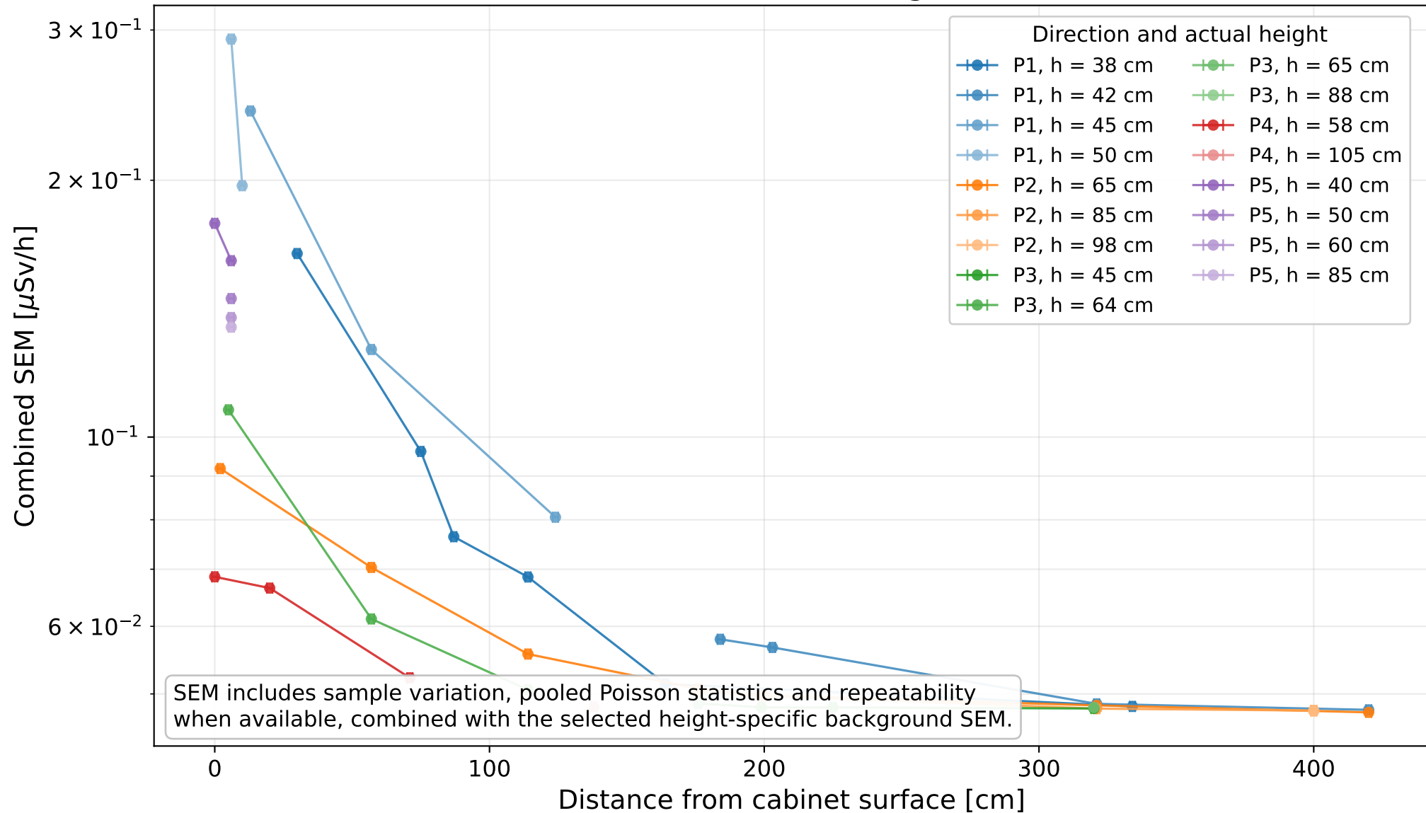
Standard error of the measured gamma indication
