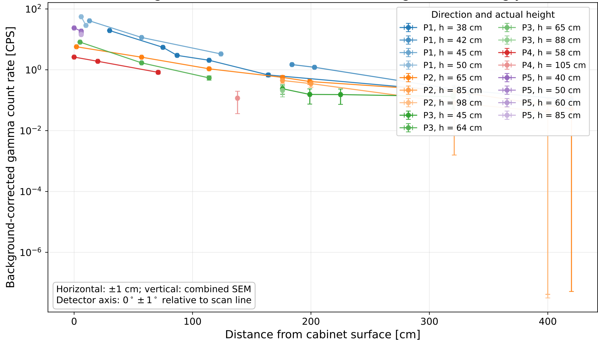
Measured gamma count rate — all detector heights — semi-log y scale
