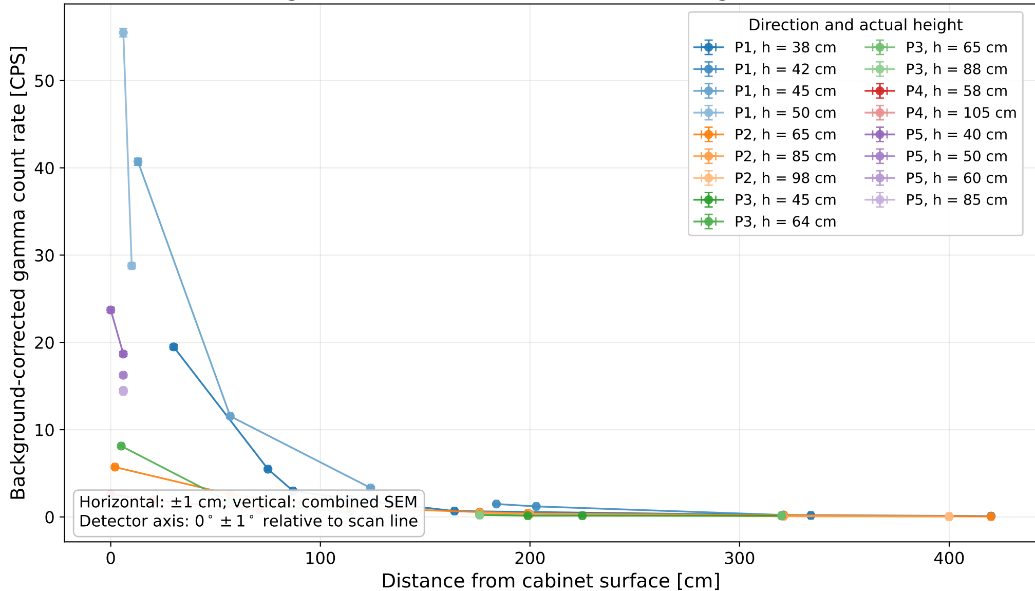
Measured gamma count rate — all detector heights — linear scale
