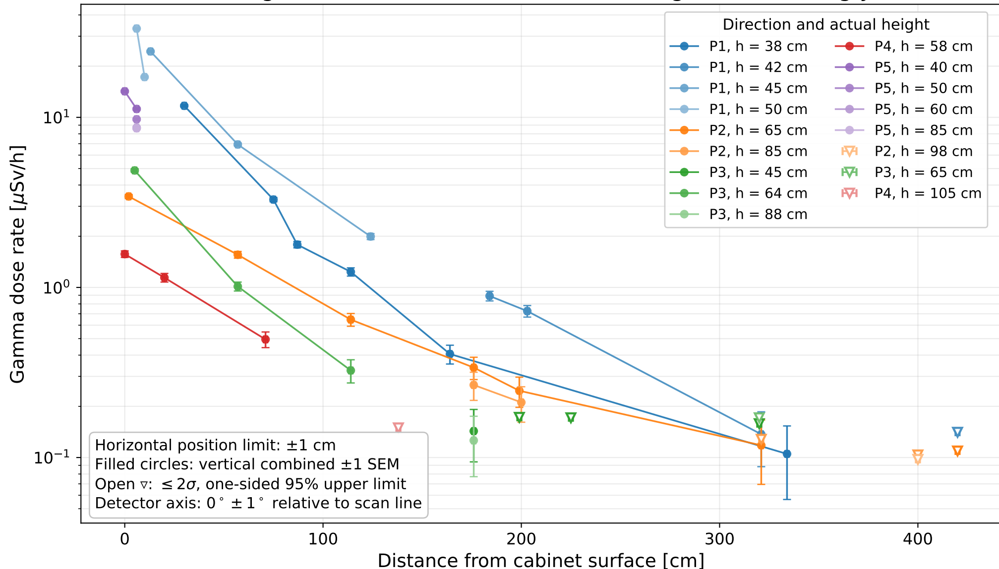
Measured gamma indication — all detector heights — semi-log y scale
