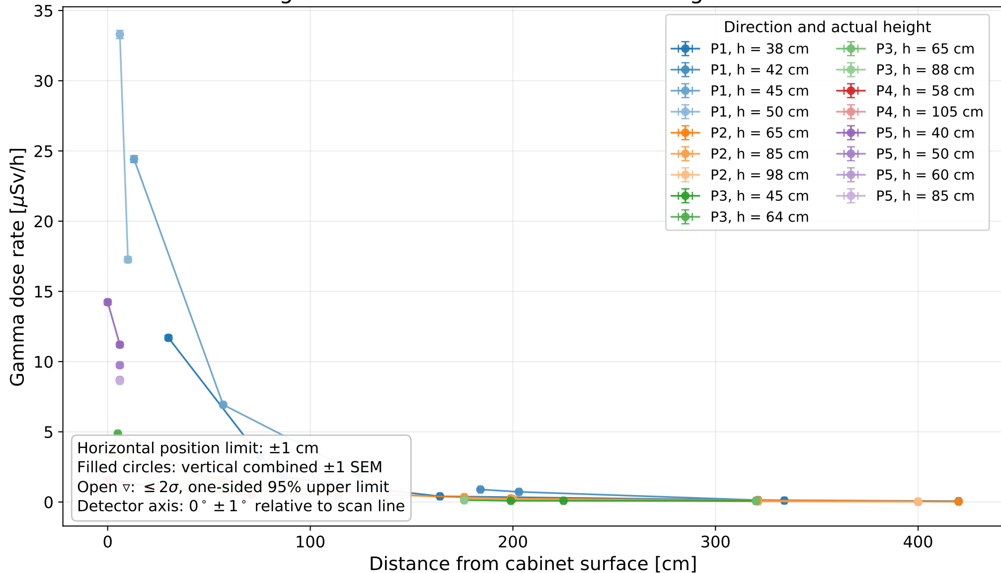
Measured gamma indication — all detector heights — linear scale
