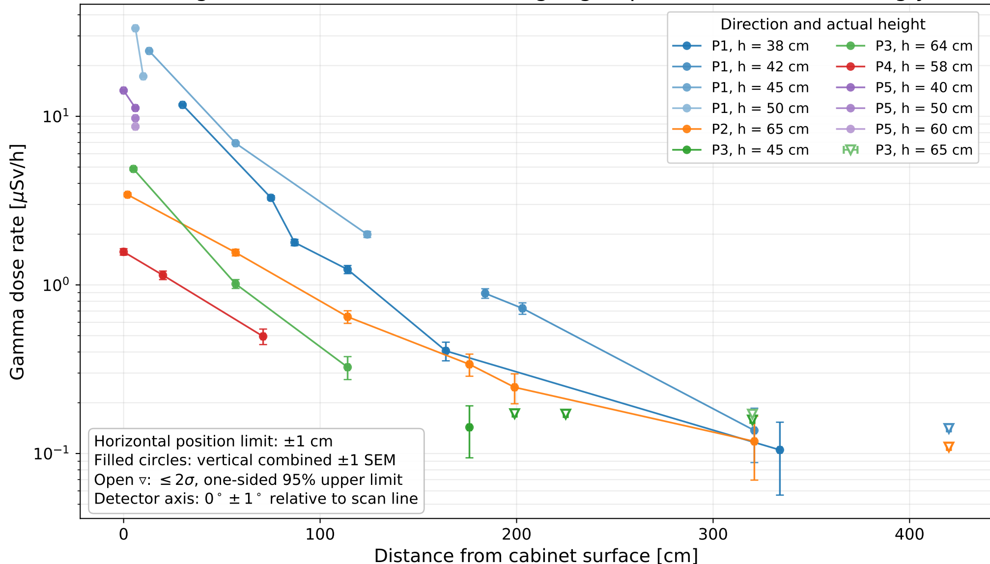
Measured gamma indication — lower height group (38–65 cm) — semi-log y scale
