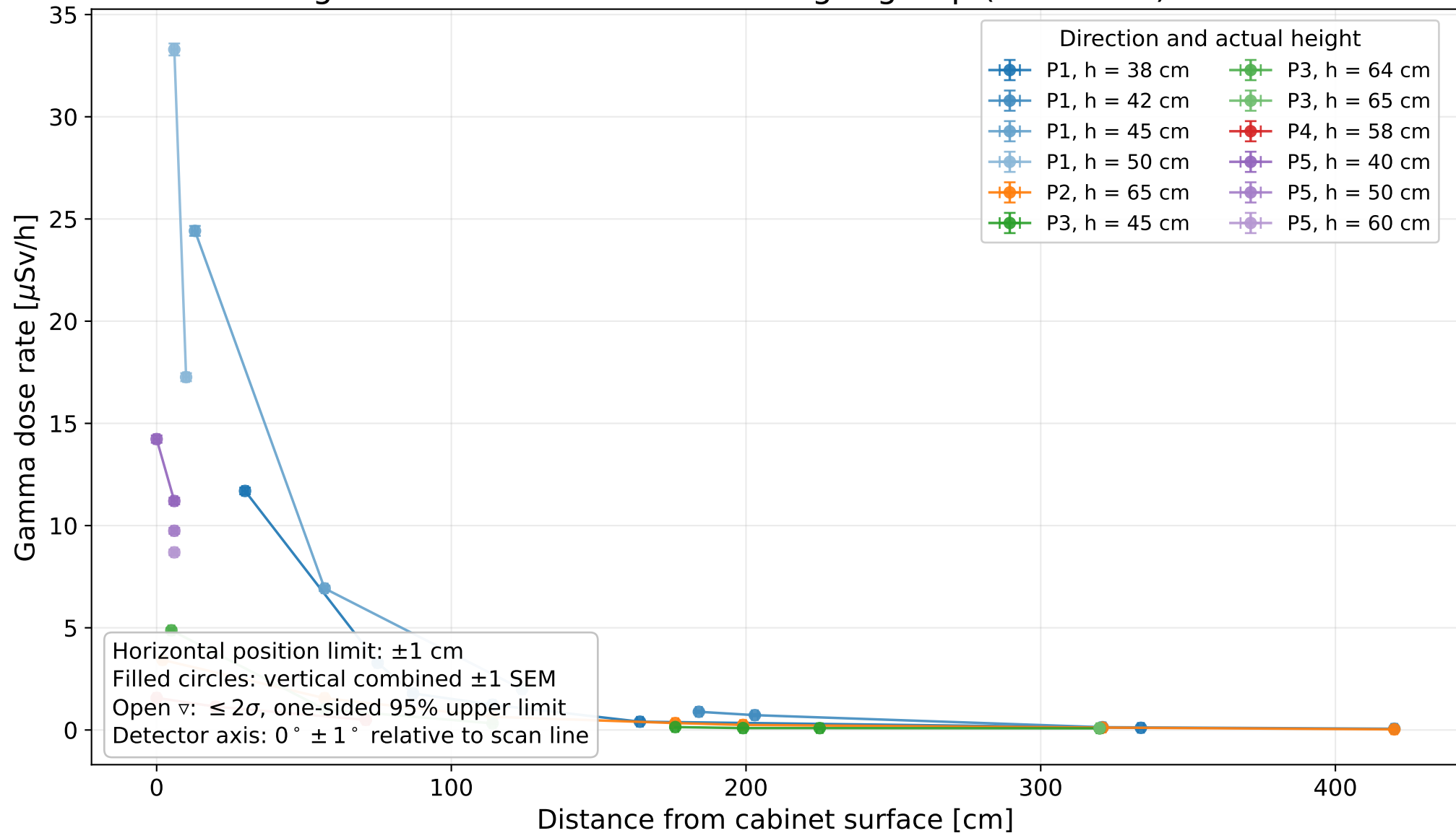
Measured gamma indication — lower height group (38–65 cm) — linear scale
