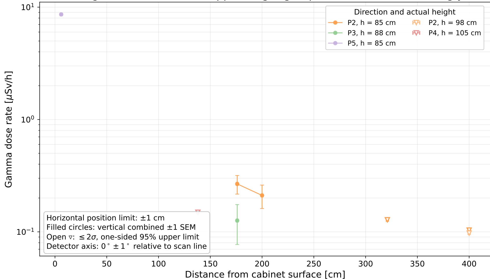
Measured gamma indication — upper height group (85–105 cm) — semi-log y scale
