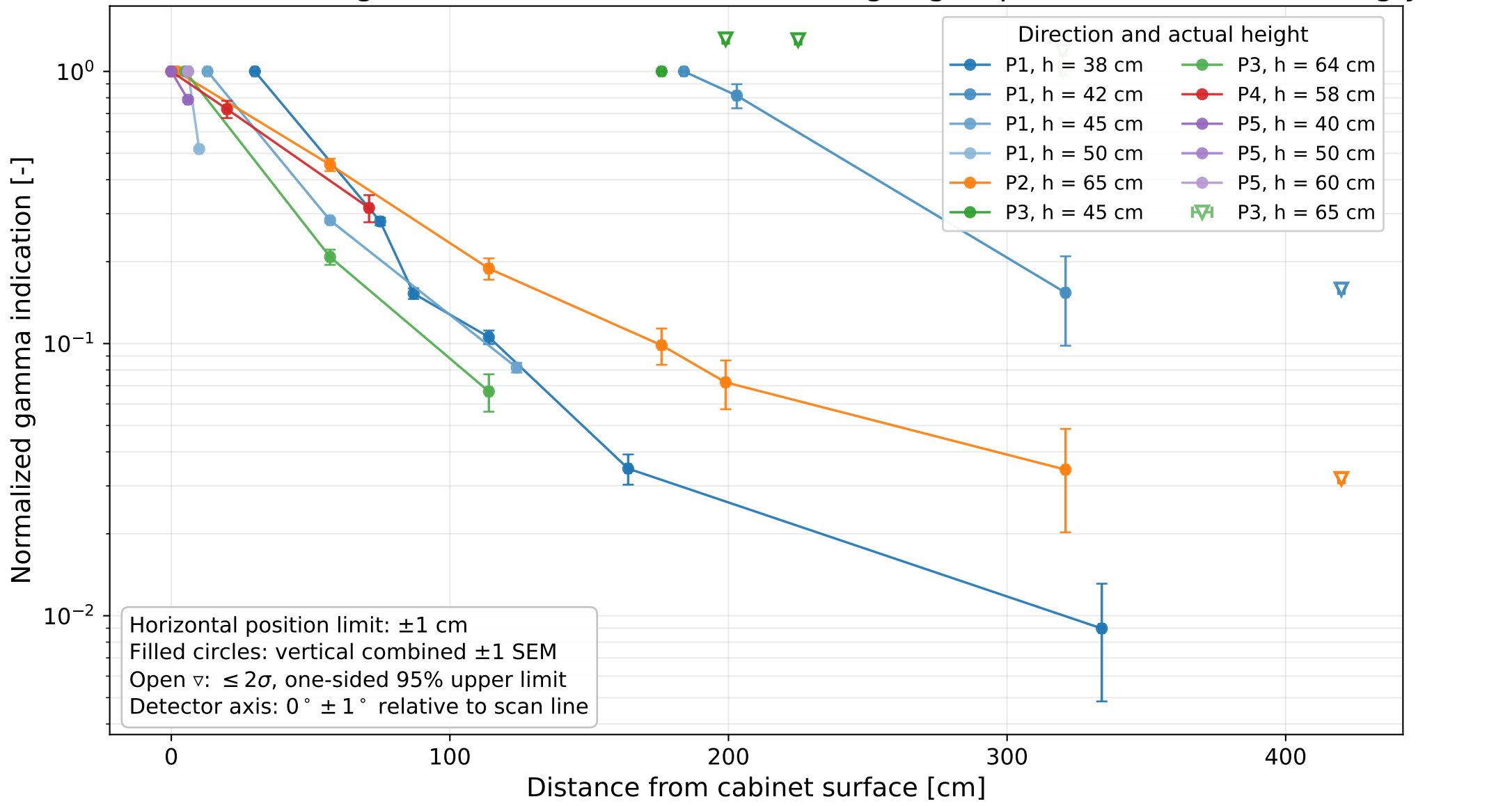
Normalized measured gamma attenuation — lower height group (38–65 cm) — semi-log y scale
