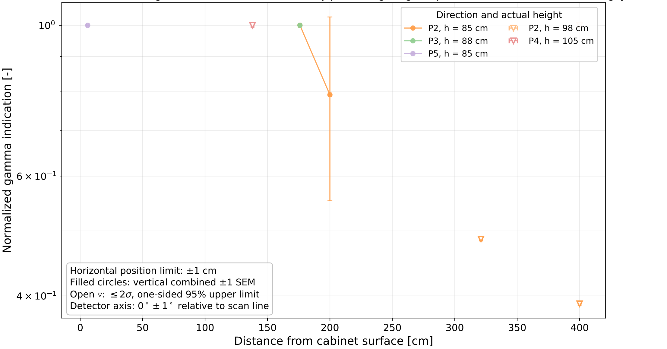
Normalized measured gamma attenuation — upper height group (85–105 cm) — semi-log y scale
