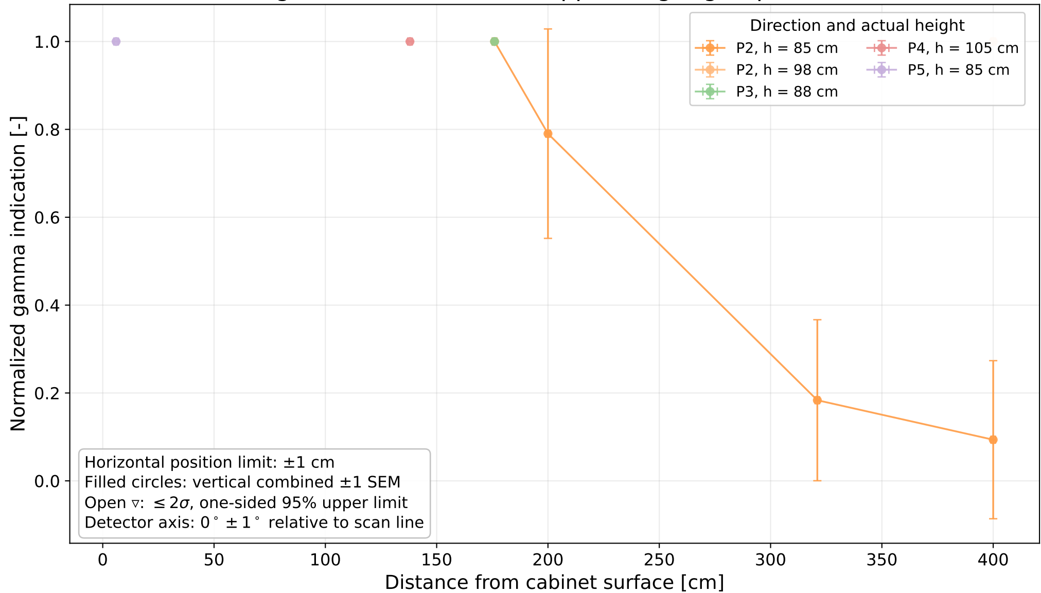
Normalized measured gamma attenuation — upper height group (85–105 cm) — linear scale
