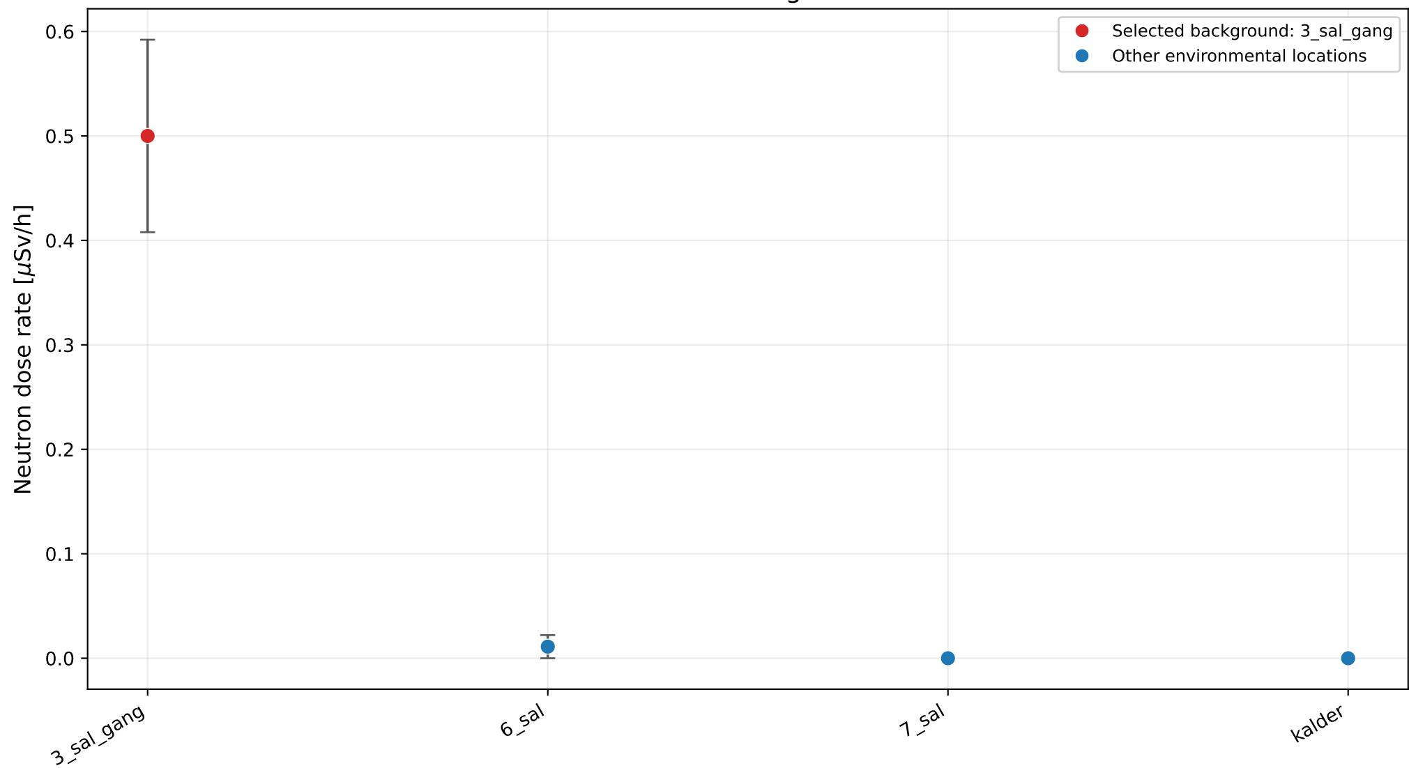
Environmental neutron-background measurements
