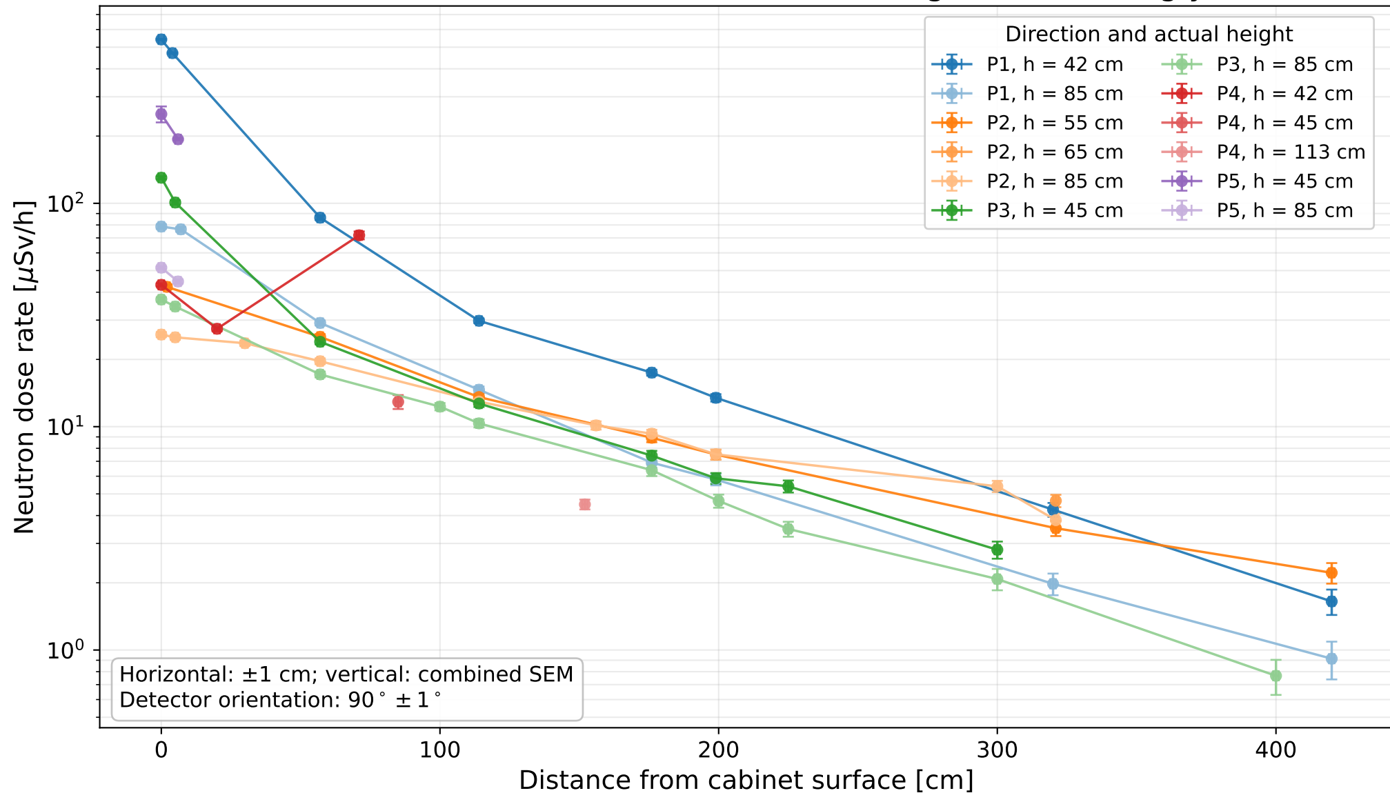
Measured neutron dose rate — all detector heights — semi-log y scale
