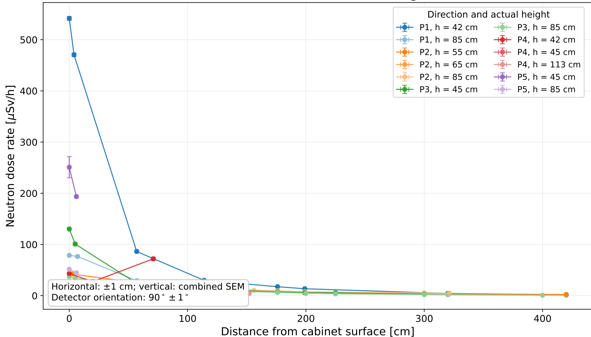
Measured neutron dose rate — all detector heights — linear scale
