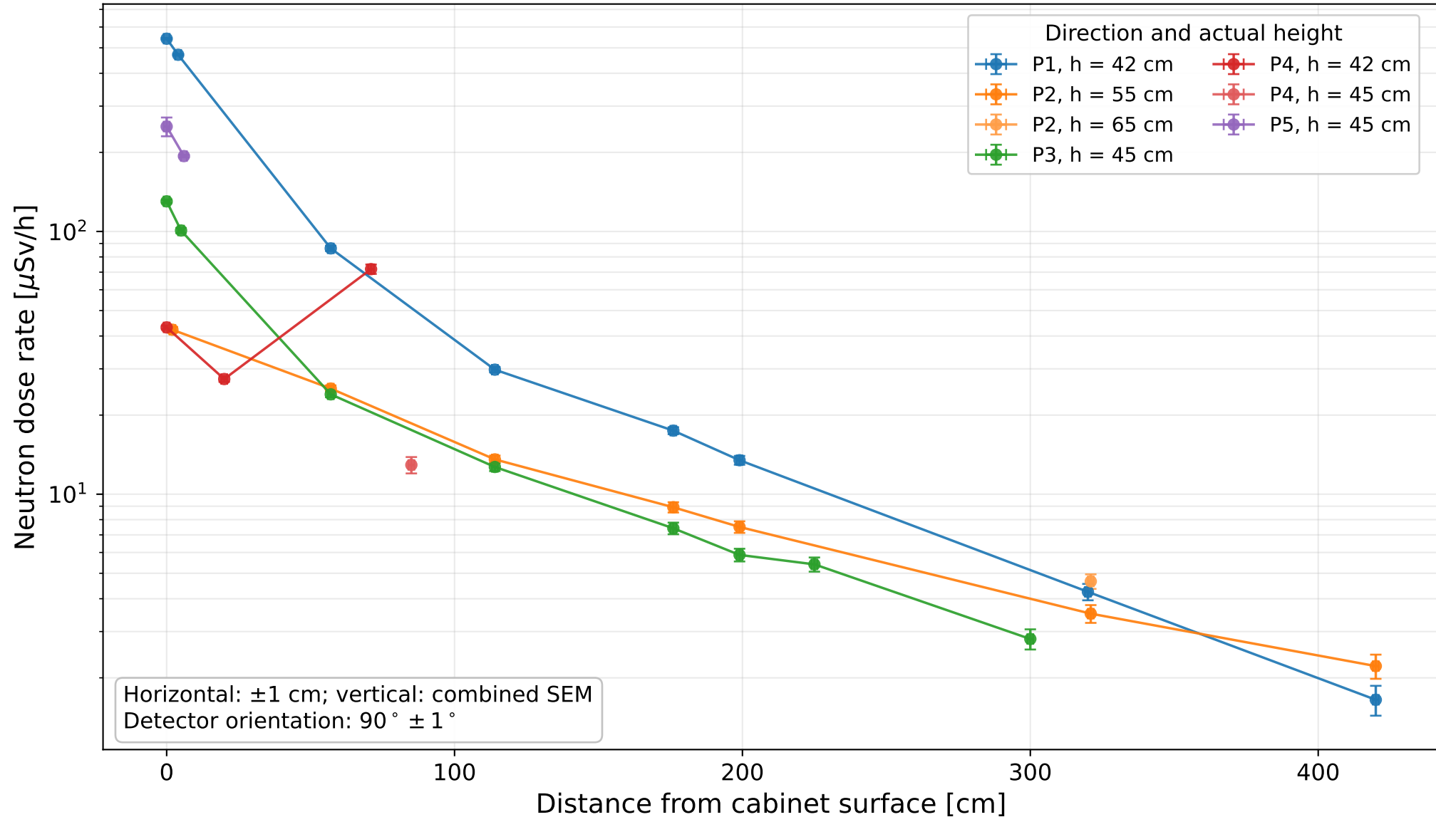
Measured neutron dose rate — lower height group (42–65 cm) — semi-log y scale
