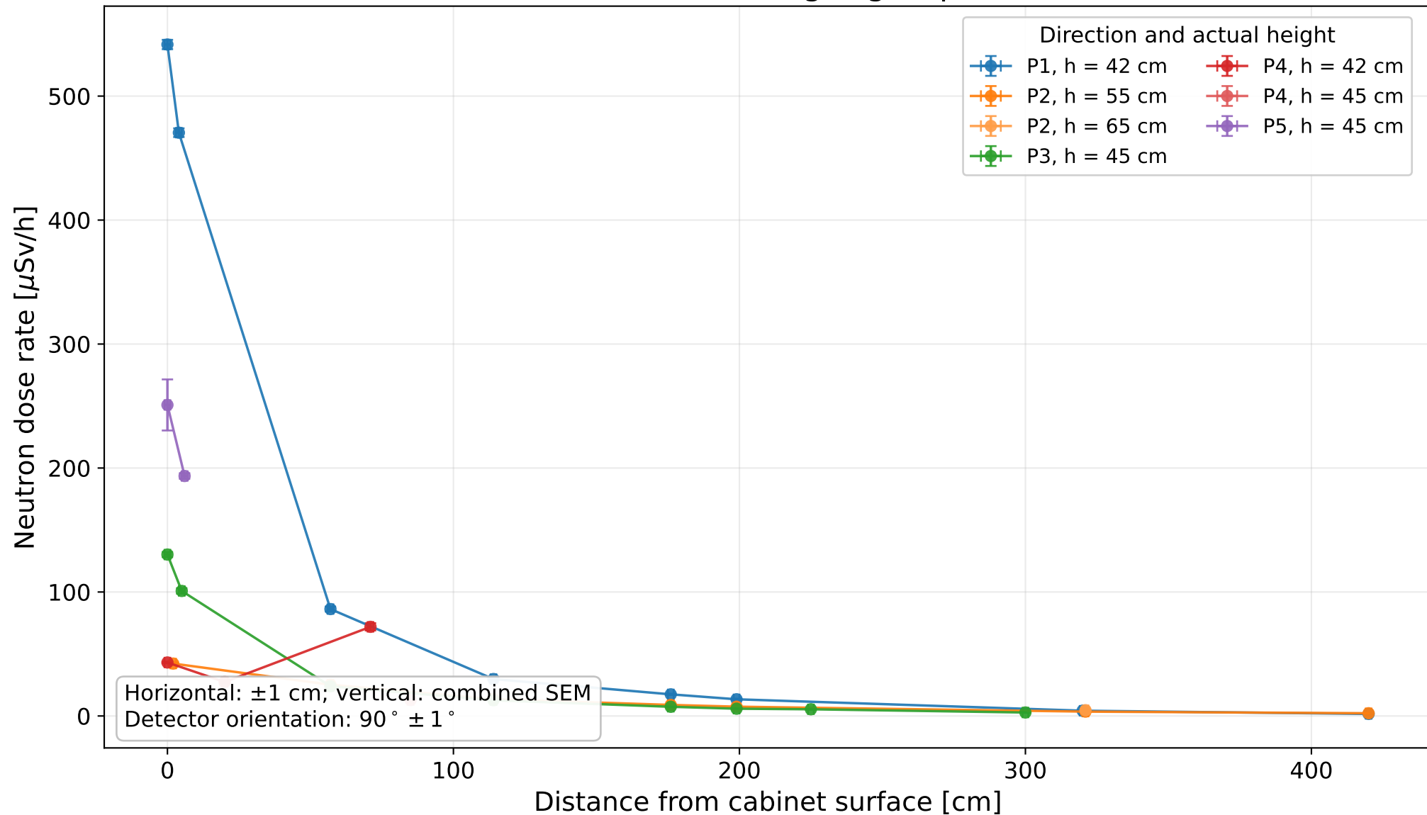
Measured neutron dose rate — lower height group (42–65 cm) — linear scale
