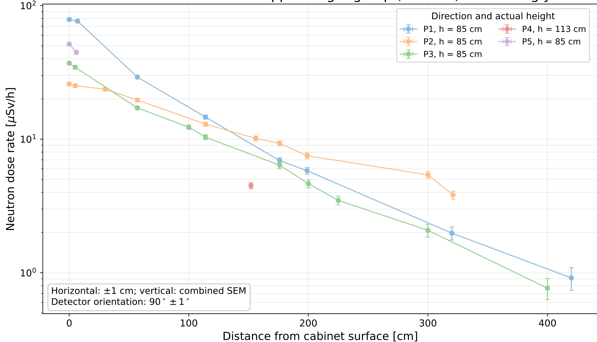
Measured neutron dose rate — upper height group (85+ cm) — semi-log y scale
