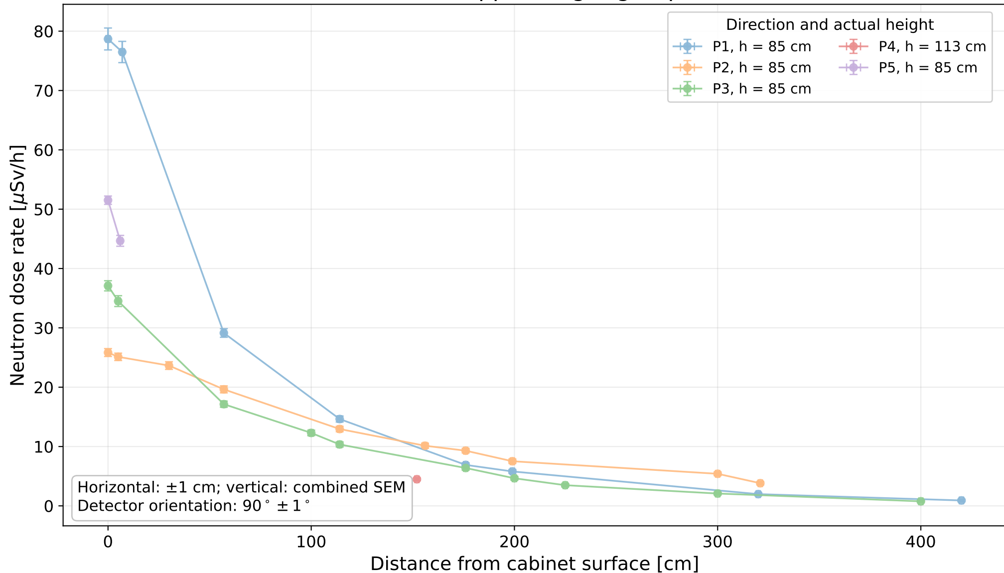
Measured neutron dose rate — upper height group (85+ cm) — linear scale
