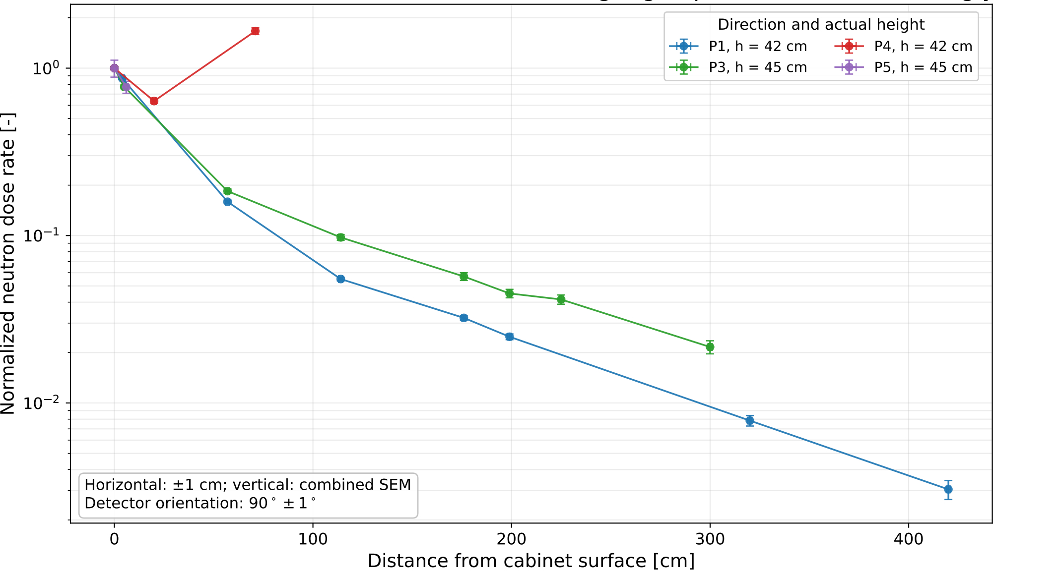
Normalized measured neutron dose rate — lower height group (42-65 cm) — semi-log y scale
