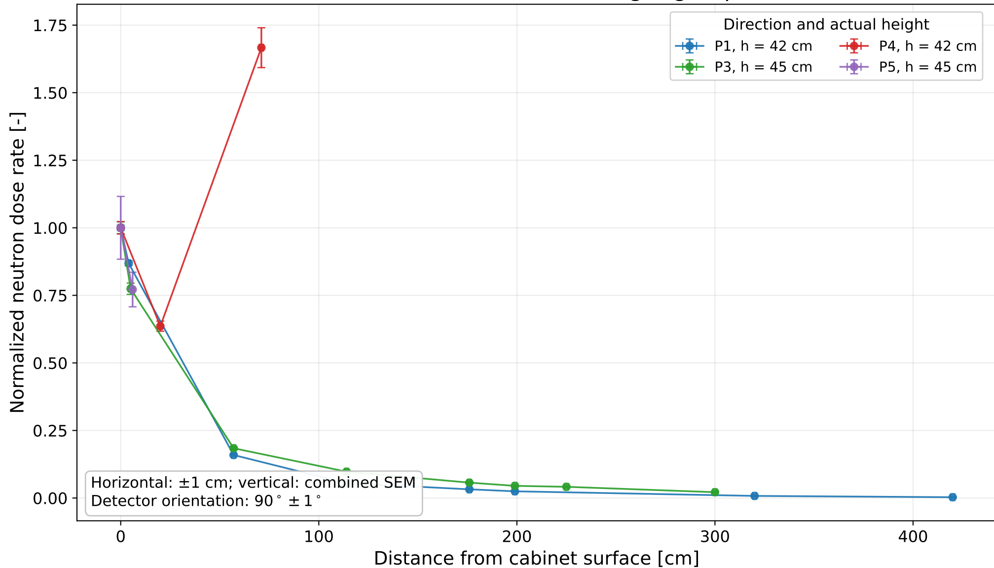
Normalized measured neutron dose rate — lower height group (42–65 cm) — linear scale
