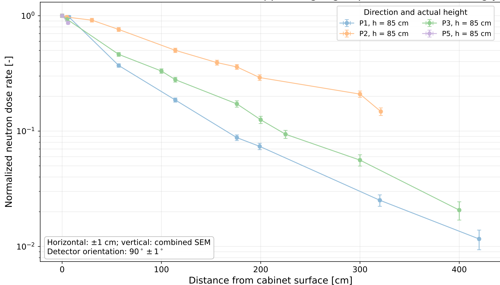
Normalized measured neutron dose rate — upper height group (85+ cm) — semi-log y scale
