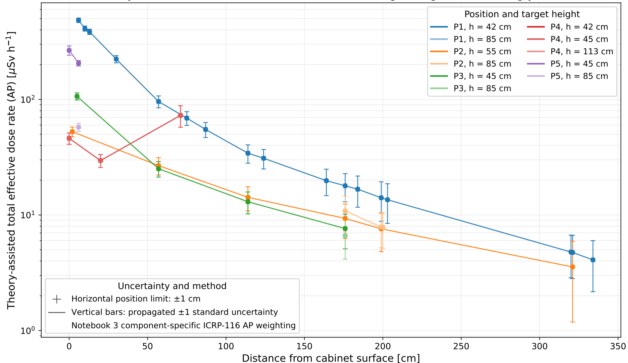
Theory-assisted measured total dose rate — all target heights — semi-log y scale
