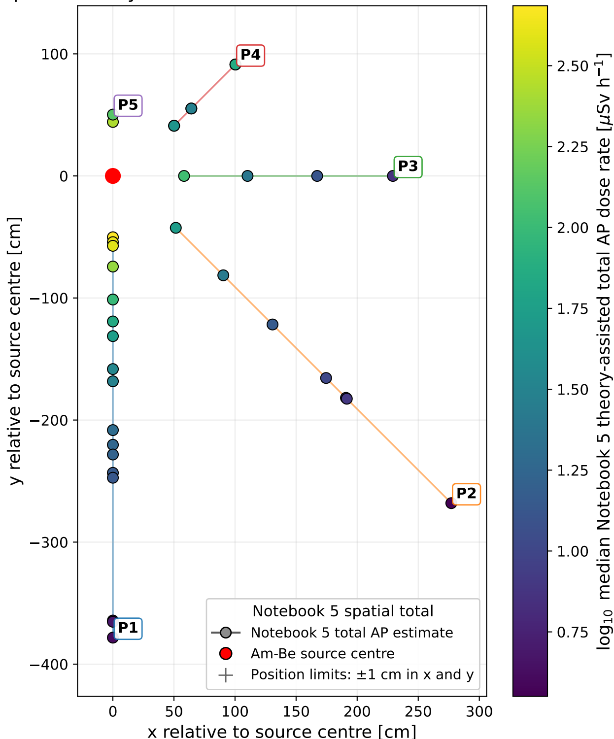
Spatial theory-assisted measured total AP dose-rate field
